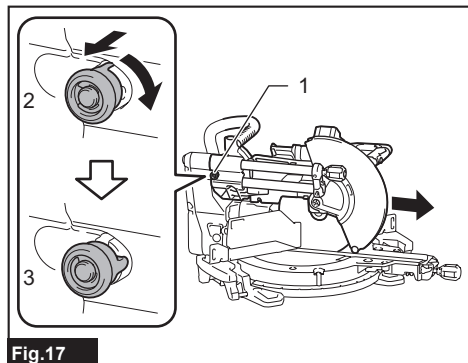
Fig.17 ► 1. Stopper pin 2. Locked position 3. Unlocked position
